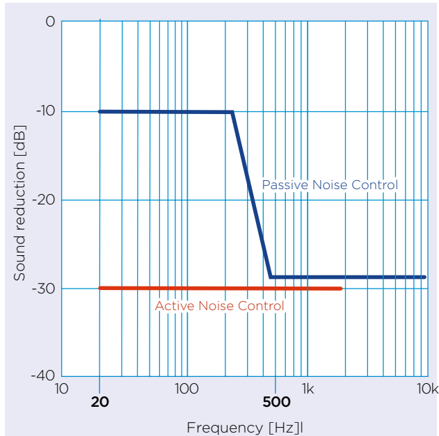
Comparison between passive and active noise control methods.
