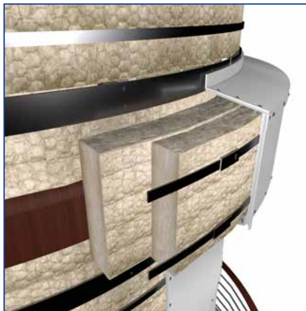
Figure 19. COLUMN DETAIL 1
